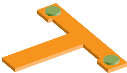
Alloys with a large pasty range enable a preassembled solderable connect.
